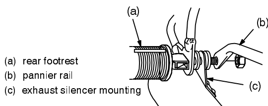
Pannier Rail Lower Mounting
