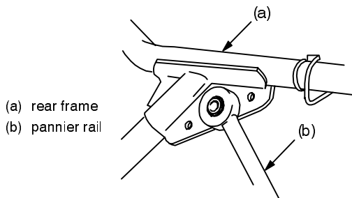
Pannier Rail Upper Mounting
